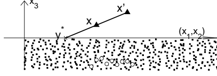
FIG. 7.1. Configuration considered in Section 7. The circles are the random sources, the bottom half-space is randomly heterogeneous, the observation points \mathbf{x} and \mathbf{x}' are in the homogeneous upper half-space, and \mathbf{y}^* is the intersection of the ray going through \mathbf{x} and \mathbf{x}' with the plane x_3=0 .
