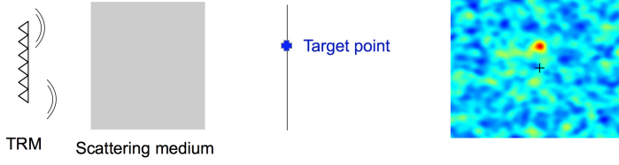
FIG. 5.1. Focusing on a prescribed point in the neighborhood of the original source location. The TRM emits the complex-conjugated recorded field with an additional linear phase (the cross in the right image stands for the original source location).
