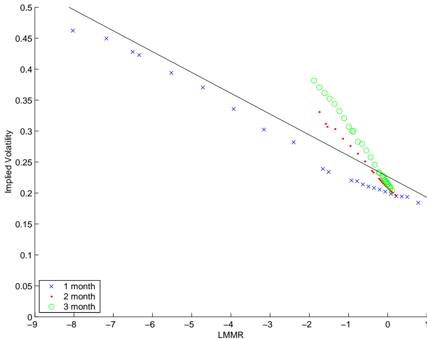
Figure 1: Implied volatility as a function of LMMR on January 12, 2000, for options with at least two and at most 93 days to maturity. The one month options expire in January, the two month in February, and so on. Notice the distinct strands for each maturity, in particular the large gap between the one-month and two-month implied volatilities. The solid line is the least-squares straight line fit over all these maturities and strikes at once.
