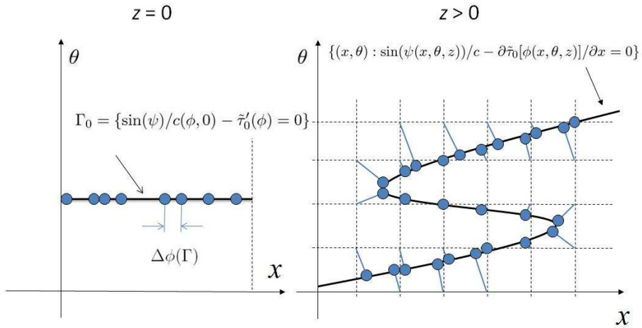
Figure 8: The sampling particles (blue dots) of the level set in the grid based particle method. Note the difference on the sampling from Fig. 2.
