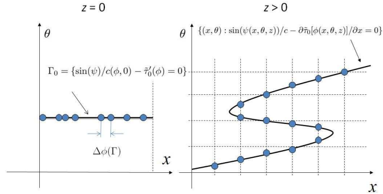
Figure 2: Eulerian Gaussian Beam with the initial wavefunction decomposed using the asymptotic decomposition. The set of sampling points \Gamma in [20, 21] are shown in blue dots. The useful level set is plotted using a black solid line.
