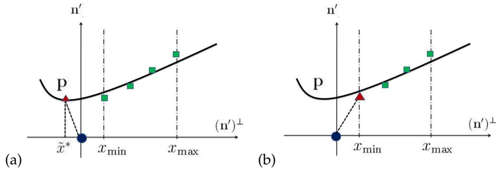
Figure 6: (a) In the original algorithm [24], any potential new foot-point (red triangle) will be rejected if x^* \notin [x_{\min}, x_{\max}] = [\min(x_j), \max(x_j)] . (b) In the new algorithm, we associate the new closest point to the closest boundary-point if the corresponding active grid point is close to the boundary. In this plot, we associate the active grid point (blue circle) to the particle corresponding to x_{\min} (red triangle) assuming it is a boundary-point.
