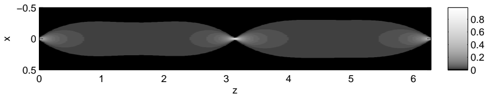
Figure 15: Diffraction of a Gaussian in a parabolic medium. The intensity I(x,z) .
