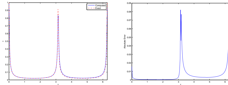
Figure 16: Diffraction of a Gaussian in a parabolic medium. (a) The intensity along x=0 , I(0,z) . The refocusing effect is clearly seen at z=\pi and 2\pi . (b) The absolute difference between the computed solution in (a) and that from the small-angle approximation.
