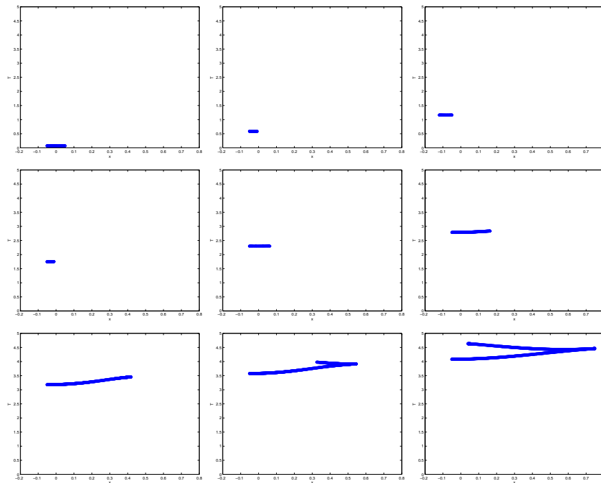
Figure 22: Diffraction of a plane wave in a sinusoidal medium. We show the arrivaltimes at various z 's. Two arrivals are clearly seen at the last two subplots.
