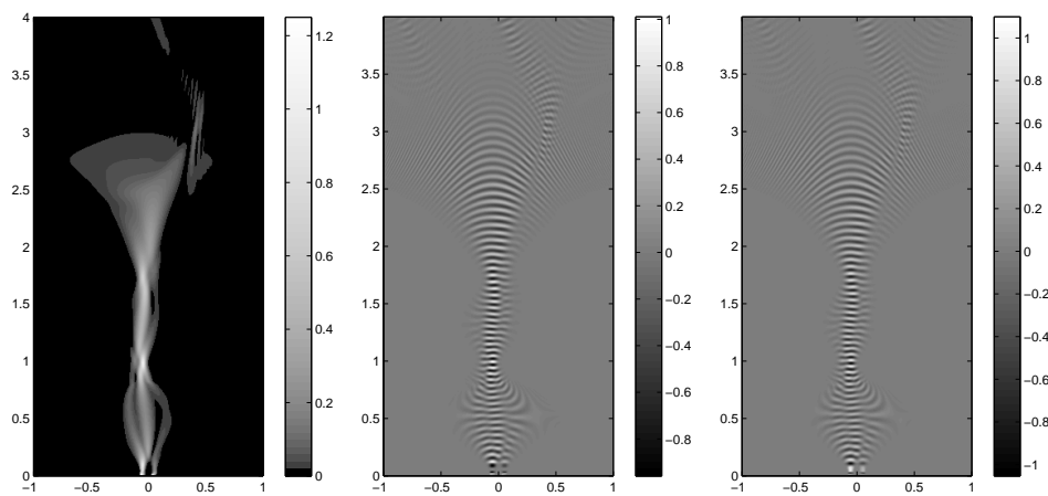
Figure 25: Diffraction of a plane wave in a sinusoidal medium. (a) The intensity of the wavefield. (b) The real part of the wavefield. (c) The imaginary part of the wavefield.
