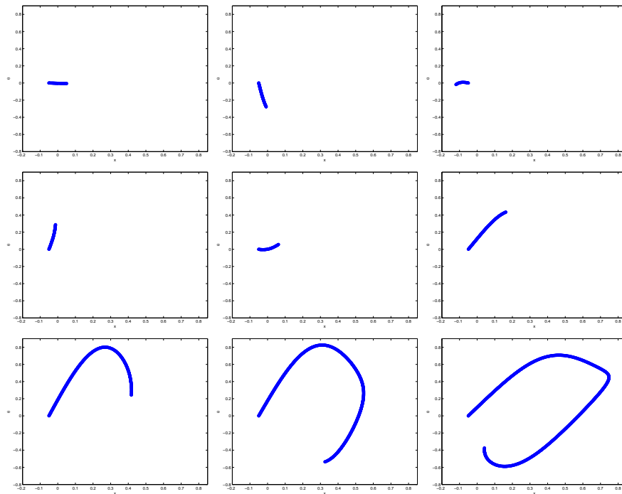
Figure 20: Diffraction of a plane wave in a sinusoidal medium. We show the evolution of the open level curve in the x - \theta phase space at various z 's. The multiple arrivals are clearly seen at the last two subplots.
