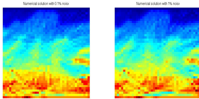
Figure 13: Marmousi model. Left: The numerical solution with 0.1% noise. The relative error is 4.16%. Right: The numerical solution with 1% noise. The relative error is 5.53%.
