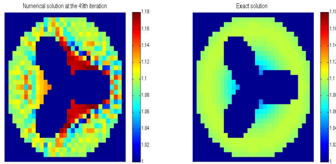
Figure 11: Left: Numerical solution at the 49-th iteration. Relative error is 2.57%. Right: Exact solution.
