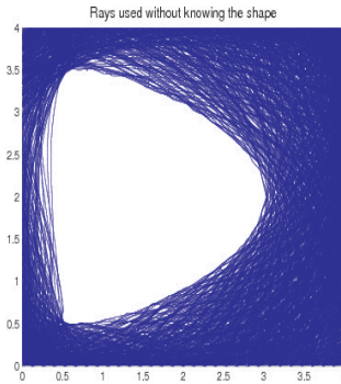
Figure 8: Ray coverage of the unknown obstacle.
