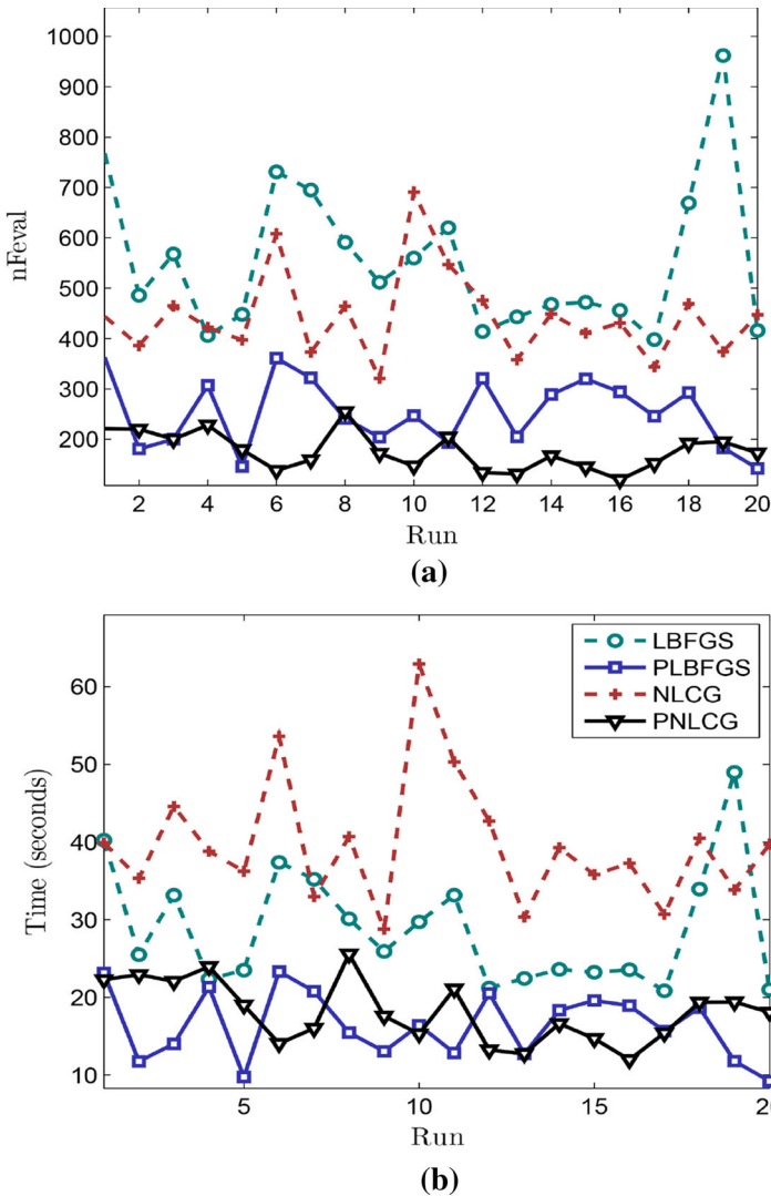
Fig. 9 20 simulations with density function \rho(x, y) = e^{-20(x^2+y^2)} + \frac{1}{20} \sin^2(\pi x) \sin^2(\pi y) on a regular hexagon bounded by [-2, 2] \times [-1.732, 1.732] . a Run versus nFeval, b run versus time
