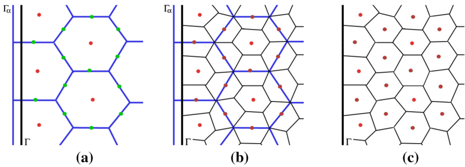
Fig. 16 Refinement of Voronoi Tessellation. a Voronoi Tessellation on the coarse grid. Green nodes are the midpoints of the interior cell edges, \Gamma_\alpha is the extend boundary, \Gamma is the original boundary. b Coarse grid and refined grid over-layed. c Refined grid truncated back to original domain
