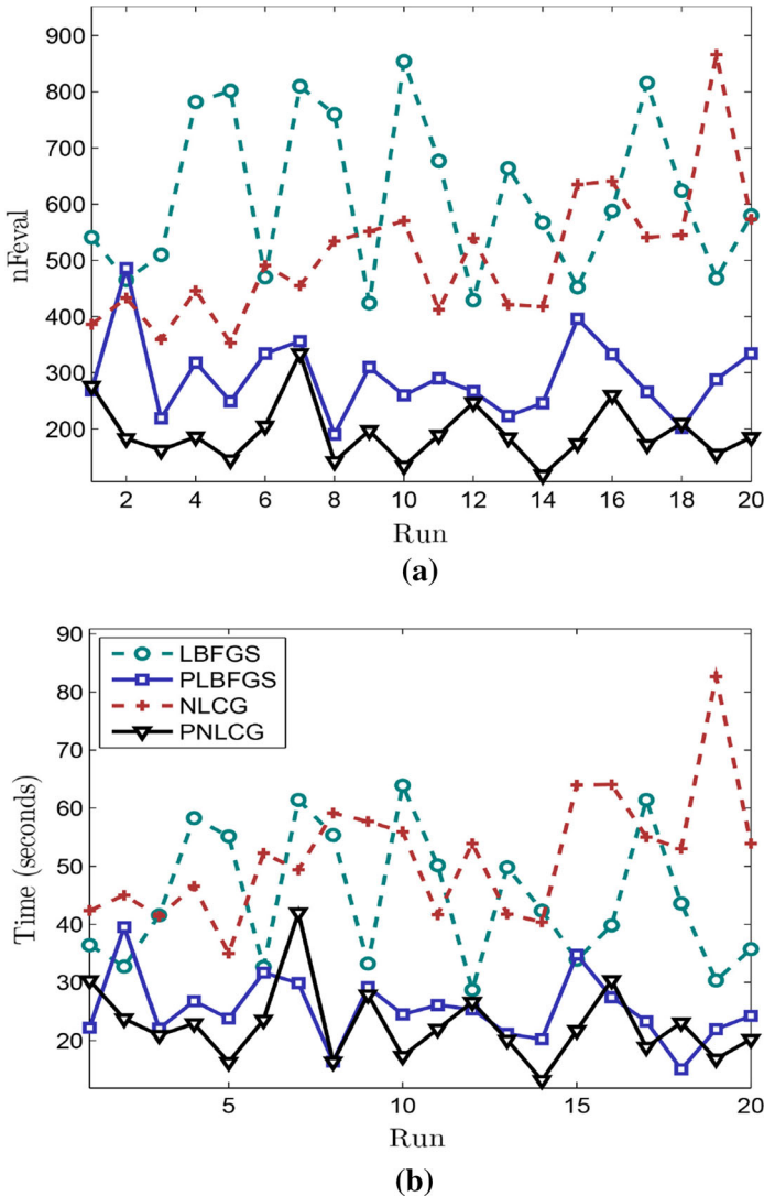
Fig. 13 20 simulations with density function \rho(x, y) = e^{-10|x^2+y^2-1|} and \Omega = (-1, 1) \times (-1, 1) . a Run versus nFeval, b run versus time
