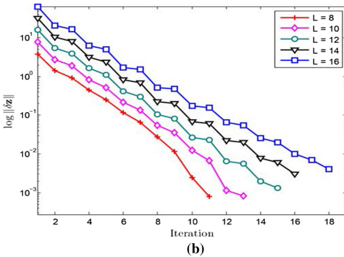
Fig. 4 Figure for error and residual for example 2, density \rho(z) = 6x^2e^{-2x^3} on (0, 2) . a Iteration versus log l_2 -norm of the weighted error. b Iterations versus log of l_2 -norm of residual
