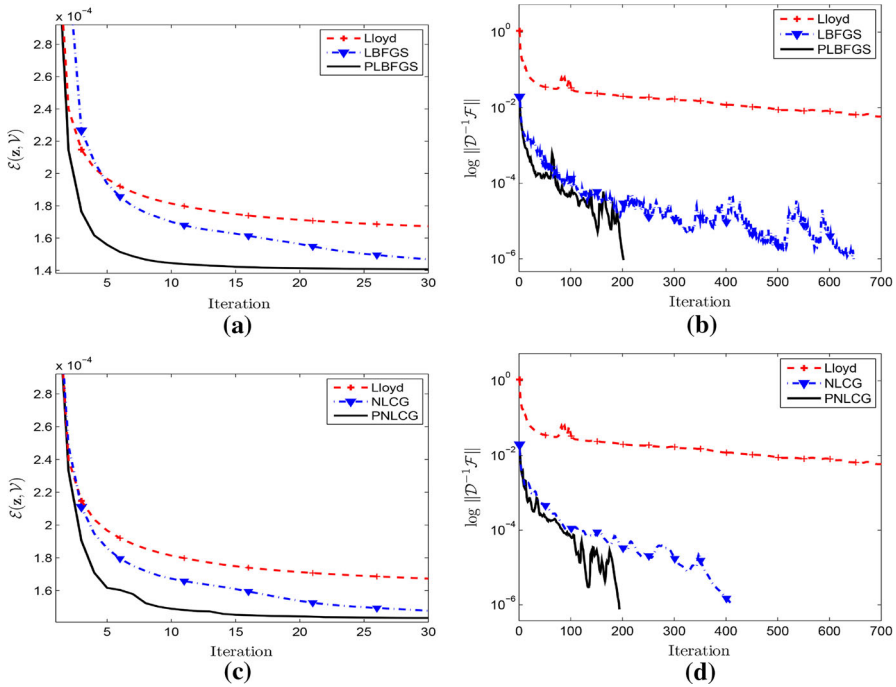
Fig. 10 Energy and error plots for example 4. a Lloyd, LBFGS(7) and PLBFGS(7) comparison of iteration versus energy, b iteration versus log of l_2 -norm weighted error, c Lloyd, NLCG and PNLCG comparison of iteration versus energy, d iteration versus log of l_2 -norm weighted error
