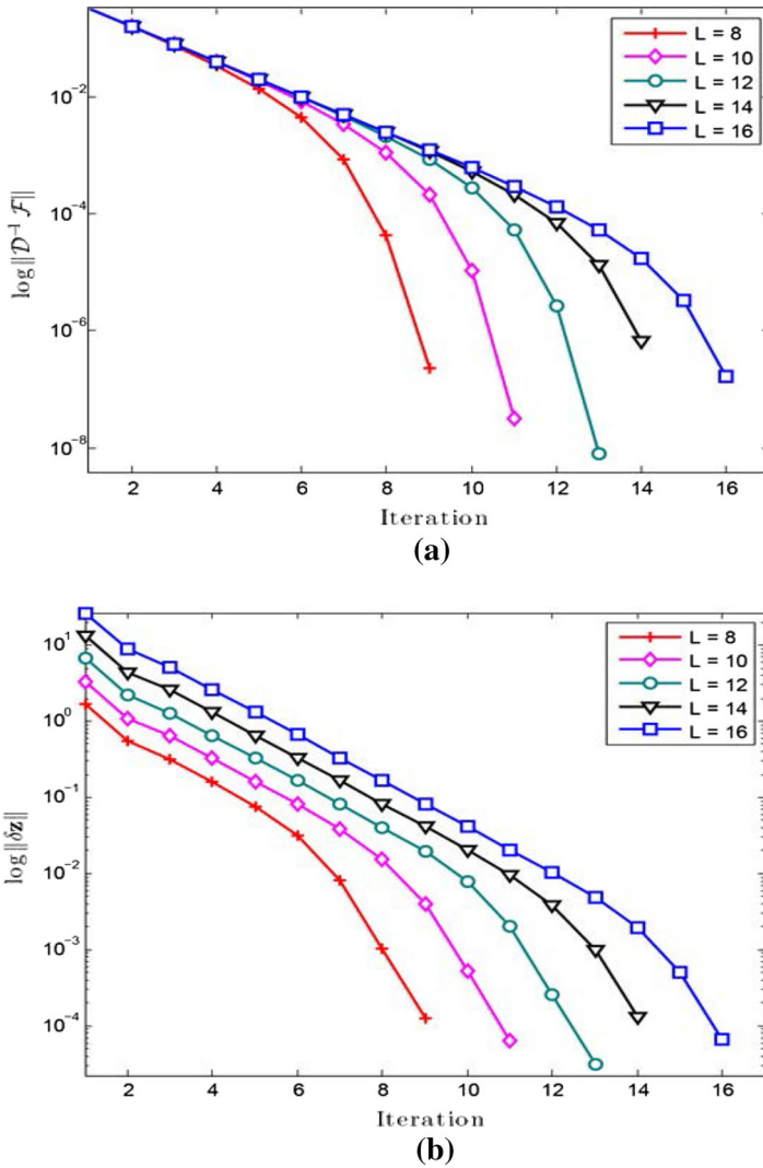
Fig. 3 Error and residual figures for example 1, density \rho(x) = e^{-10x^2} on (-1, 1) . a Iteration versus log of the l_2 -norm of weighted error. b Iterations versus log of l_2 -norm of residual
