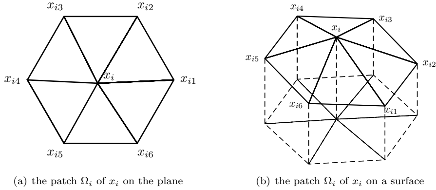
FIG. 4.1. Local patches on planar meshes and surface meshes.
