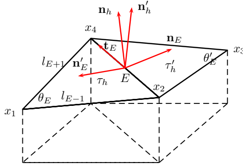
FIG. 3.1. The patch \Omega_E of the edge E .
