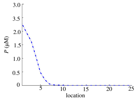
Figure 15. The mean concentration of P for the base values of all parameters.
