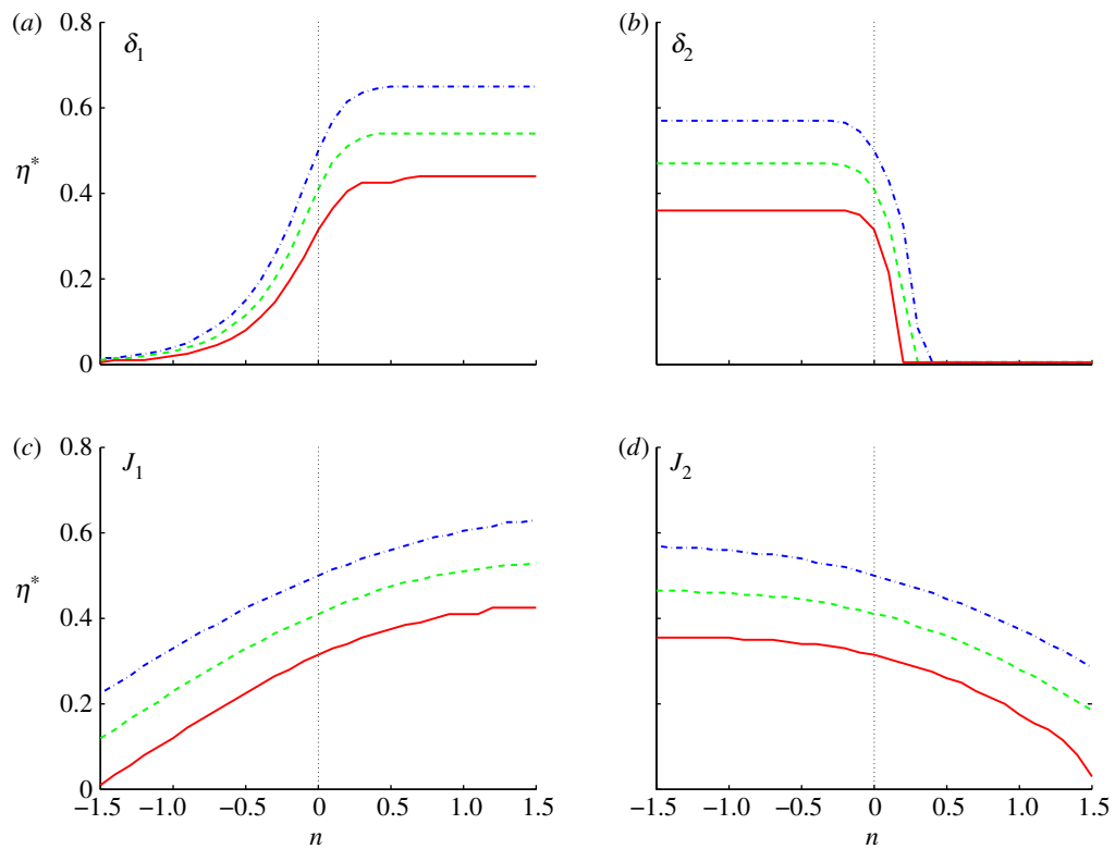
Figure 13. The variations of the boundary locations as the (a,b) flux ( \delta_1, \delta_2 respectively) and (c,d) dimensionless diffusion coefficient ( J_1, J_2 respectively) are varied in the activator–inhibitor signalling system. The y -axis is the scaled compartment number and the x -axis indicates how we vary the parameters. (a) \delta_1=10^{n-2} ; (b) \delta_2=10^{n-2} ; (c) J_1=10^{n+3} ; (d) J_2=10^{n+3} .
