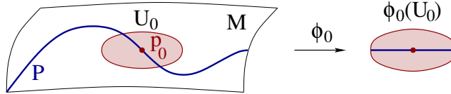
Figure 2.5: A coordinate chart adapted to a submanifold.
