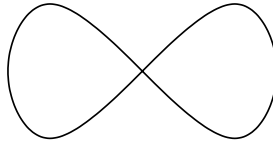
Figure 2.6: A proper immersion.
