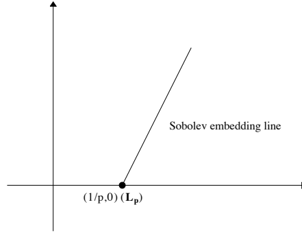
FIGURE 1. Sobolev embedding
