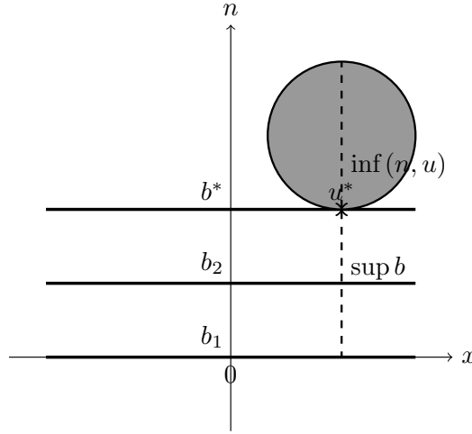
FIGURE 3. Duality.
