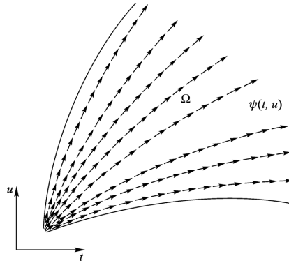
FIGURE 5. Direction field
