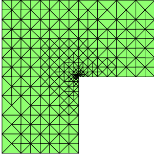
(a) Adaptive coarse mesh \mathcal{T}_0
