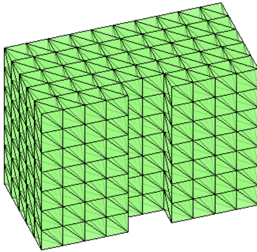
FIG. 5.2. A coarse mesh used for Example 5.4
