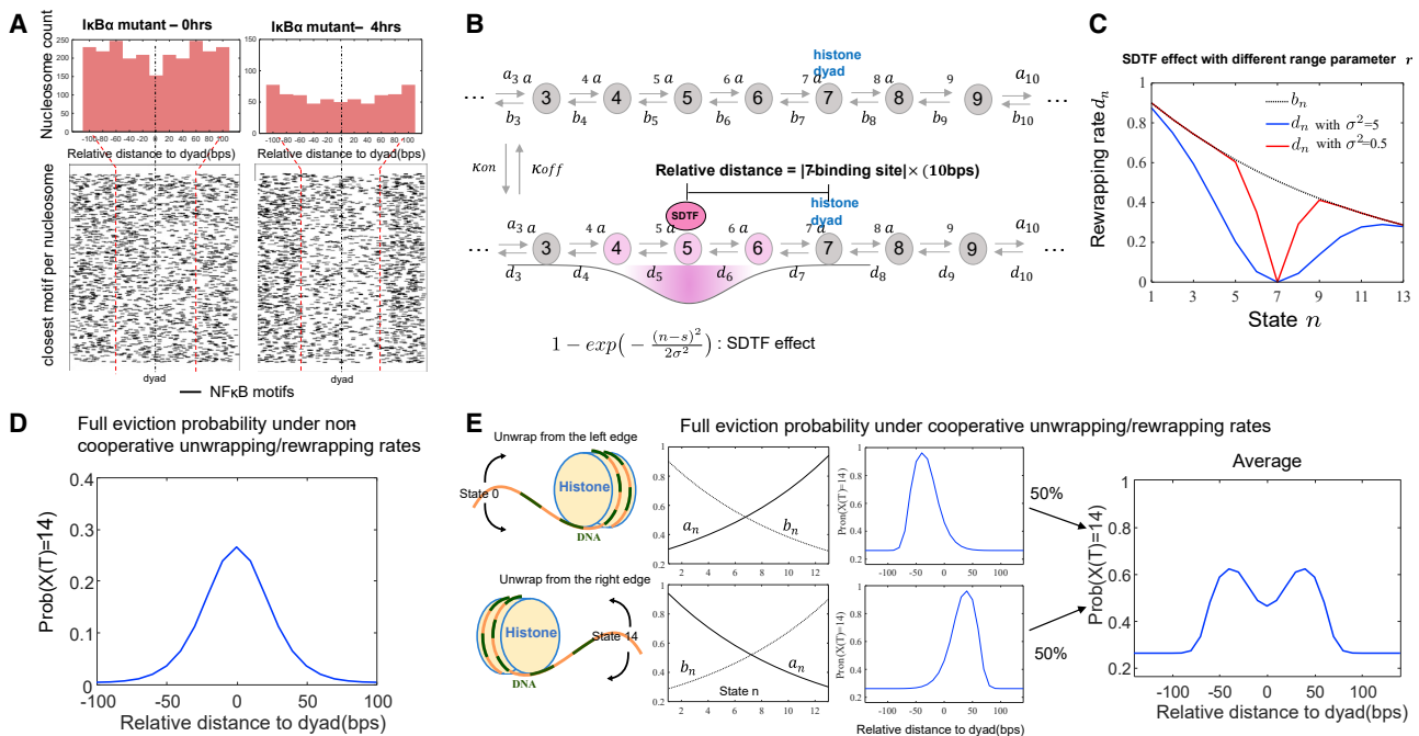
Figure 3. Modeling SDF binding sites, range of SDF effect, and cooperativity in unwrapping steps reveals potential eviction probability profiles
