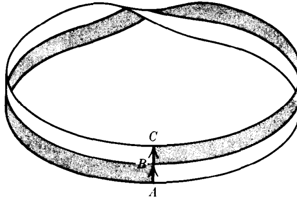
FIGURE 1.1. Constructing a Möbius strip.
