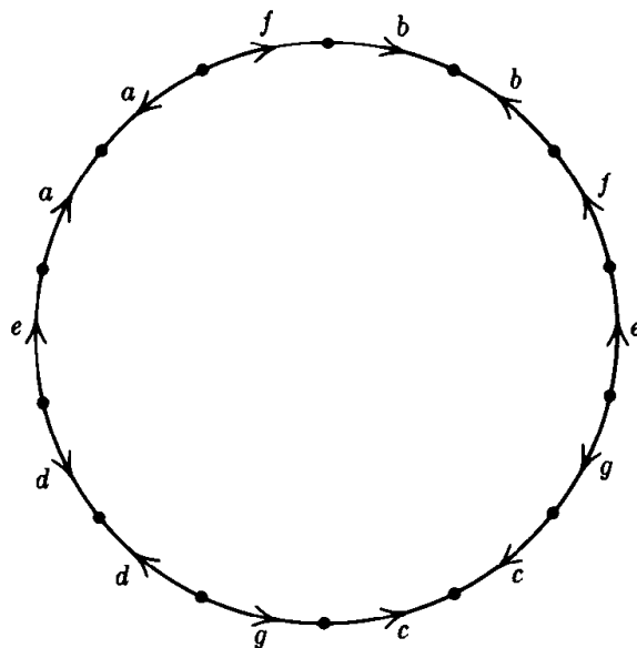
FIGURE 1.16. Simplified version of polygon shown in Figure 1.15.
