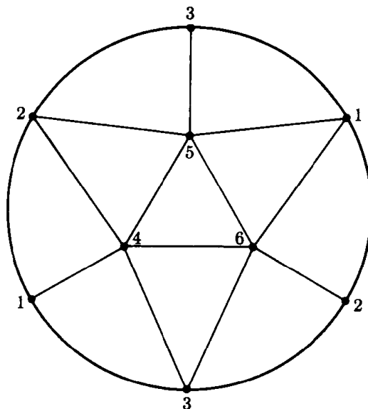
FIGURE 1.13. A triangulation of the projective plane.
