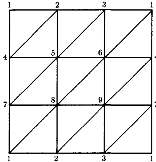
FIGURE 1.14. A triangulation of a torus.
