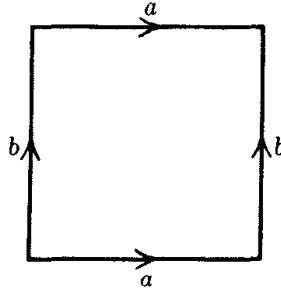
FIGURE 1.2. Construction of a torus.
