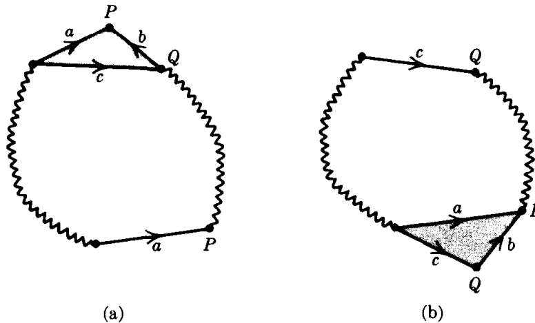
FIGURE 1.18. Third step in the proof of Theorem 5.1.
