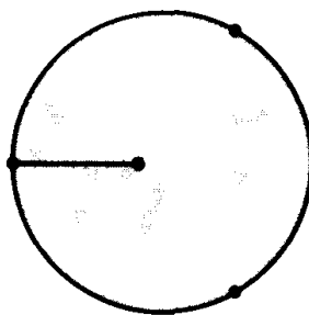
FIGURE 1.27. An allowable kind of edge.
