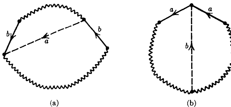
FIGURE 1.19. Fourth step in the proof of Theorem 5.1.
