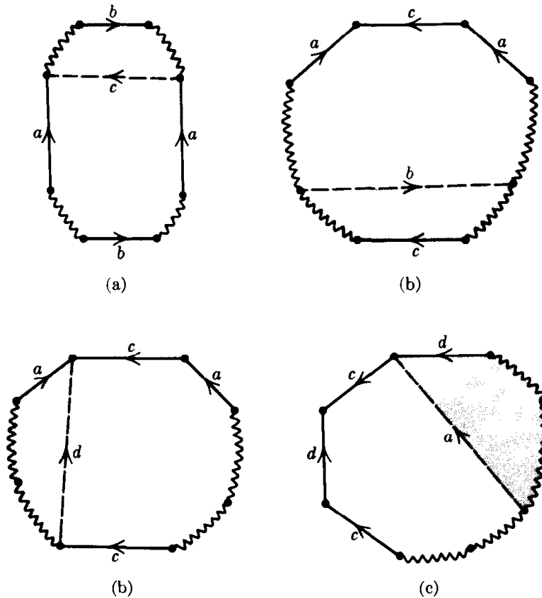
FIGURE 1.21. Fifth step in the proof of Theorem 5.1.
