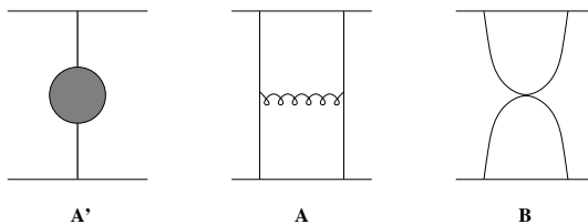
Figure 1: Two-point Feynman diagrams.
