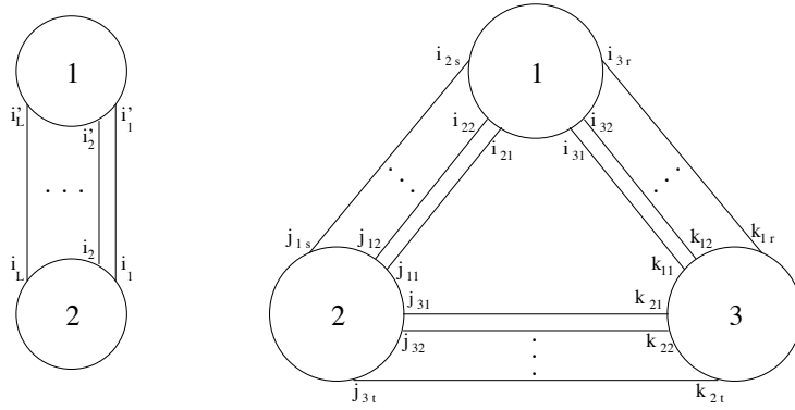
Figure 4: Labeling of the free two- and three-point operators.
