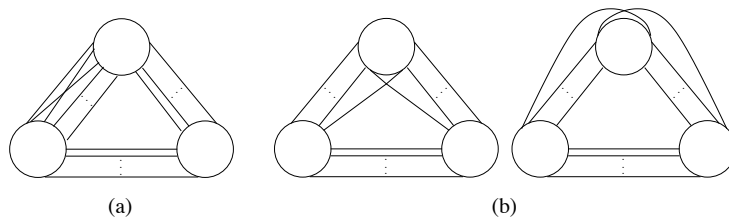
Figure 5: Examples of planar diagrams contributing to c_{123}^1 . (a) A two-point B type diagram. (b) Two three-point F type diagrams.
