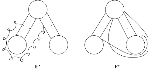
Figure 6: Non-nearest neighbor diagram for extremal three-point functions.
