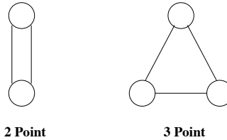
Figure 3: Free Feynman diagrams of the Konishi operator.
