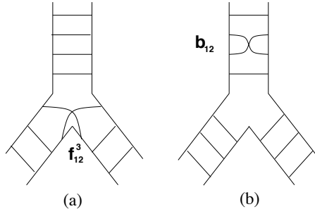
Figure 9: Zoom-up of one of the two interaction points P_{1,2} . (a) Three-point interactions f_{jk}^i are localized at the interaction points. (b) Two-point interactions b_{ij} are along the overlapping segments.
