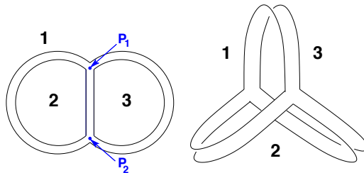
Figure 8: Witten type three-string vertex in closed string field theory. The two interaction points P_{1,2} are the analogues of the mid-point in open string field theory.
