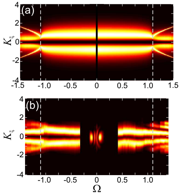
FIG. 4: (color online) (a) Same as for Fig.3 but computed for |\tilde{p}|^2 + |\tilde{p}^*|^2 . The vertical dashed line separates the snake ( \Omega < 1.08 ) from the oscillatory snake ( \Omega > 1.08 ) regimes. (b) Experimental results.
