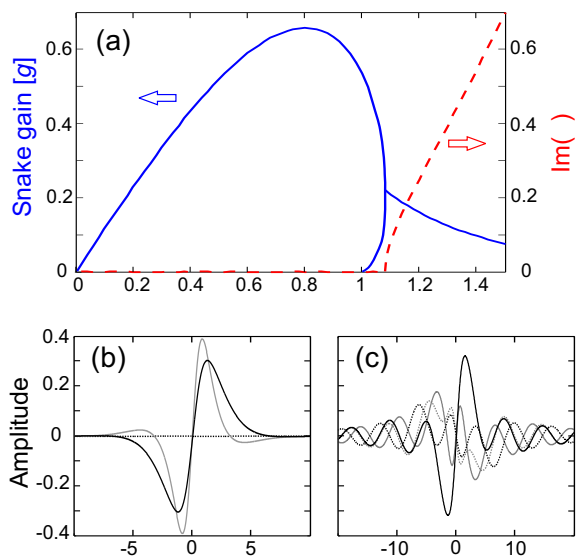
FIG. 1: (color online) (a) Snake instability gain g = 2\text{Re}(\Gamma) (solid blue line) and imaginary part of \Gamma (dashed red line) plotted as a function of the perturbation frequency \Omega . Beyond the frequency cut-off \Omega_c \approx 1.08 , \Gamma is complex and the snake instability becomes oscillatory. (b)-(c) Eigenfunctions U (gray) and V (black) plotted as a function of the transverse coordinate \xi below (b) and above (c) \Omega_c . Dashed lines stand for the real part and solid lines for the imaginary part. Figures adapted from [5].
