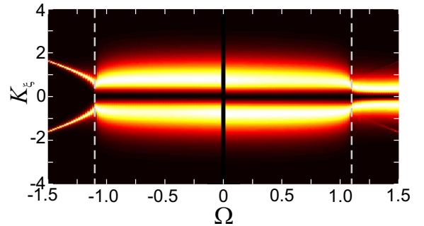
FIG. 3: (color online) Density plot of the theoretical evolution of the angularly resolved spectrum |\tilde{p}|^2 as a function of the frequency \Omega . Each spatial spectra (i.e. each profiles for a given frequency \Omega ) has been normalized to unity. Brighter colors stand for larger amplitudes. The vertical dashed lines separate the snake ( \Omega < 1.08 ) from the oscillatory snake ( \Omega > 1.08 ) regimes.
