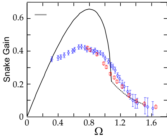
FIG. 2: (color online) Snake gain as a function of the normalized frequency perturbations \Omega , experimentally recorded for two different slab waveguides (blue diamonds and red squares). The solid and dashed lines show the theoretical snake and oscillatory snake gains, respectively. The length of the gray thick line displayed in the upper left corner gives the spectral width of the soliton and the seed input beams.
